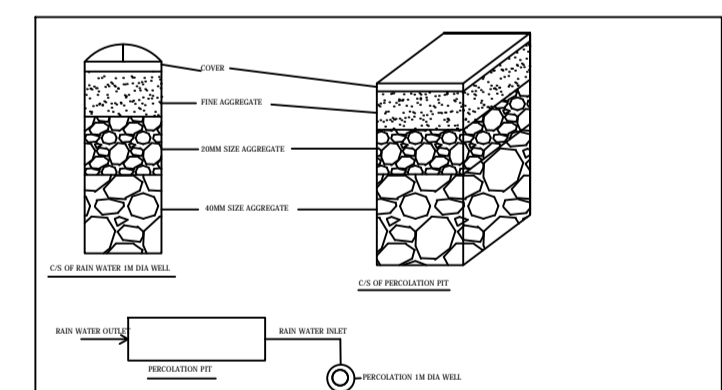
DETAILS OF RAIN WATER HARVESTING
